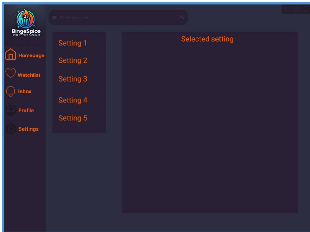
Settings Mockup
