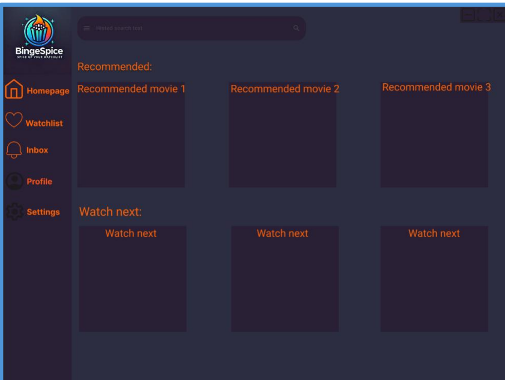
Homepage Mockup
